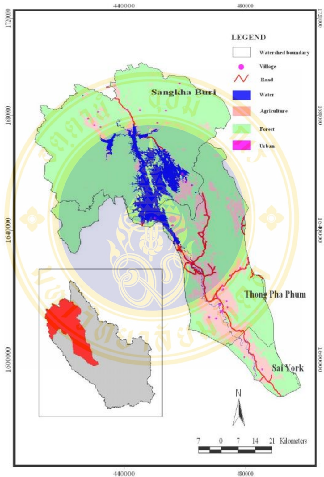
Figure 4.14: Location of Village in the Khwai Noi Upper River Source: Land Use Map, Scale 1:50,000, DLD (2000).
