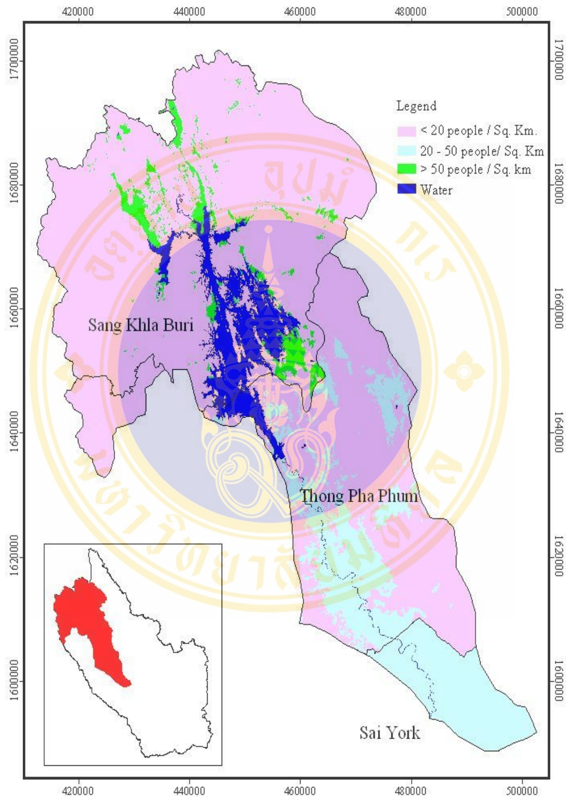
Figure 5.11: Population Density in the Khwai Noi Upper River
