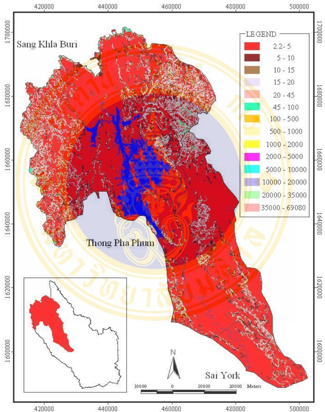
Appendix D-3: The LS layer of the Kwai Noi Upper River
