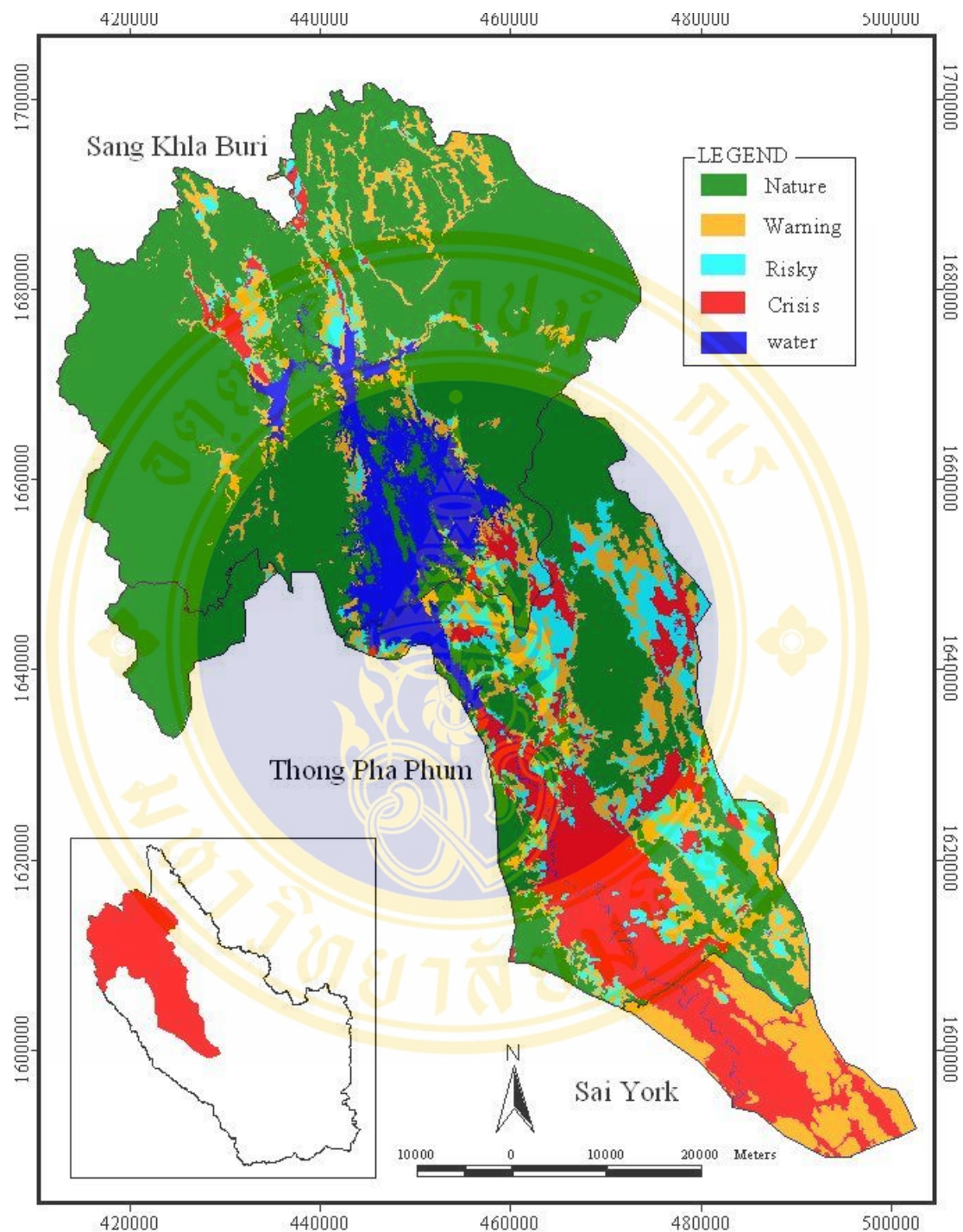
Figure 5.12: Watershed Situation in the Upper River Khwai Noi Based on Year 2000
