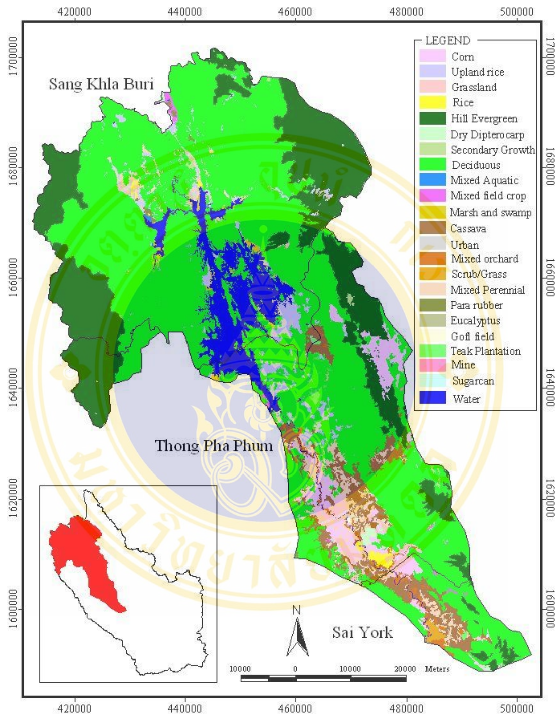
Figure 5.5 Land Use Classification with Crop Pattern in the Khwai Noi Upper River
