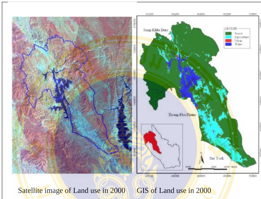
Figure 5.1: The Comparison of Land Use Change in the Khwai Noi Upper River between 1990, 1995 and 2000 (Cont.)
