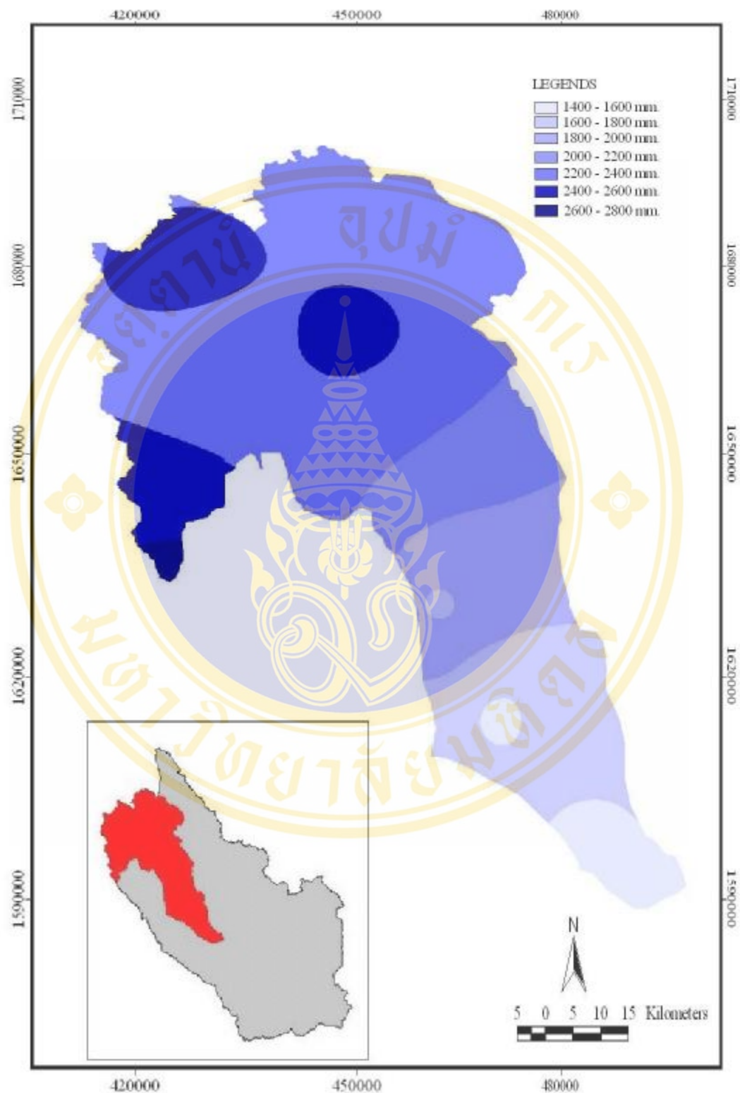
Figure 5.8 Annual Rainfall Map of the Khwai Noi Upper River
