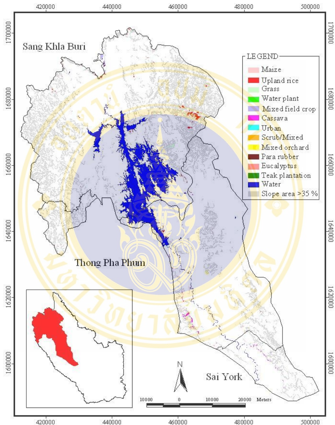
Figure 5.10: Land Utilization within Slope greater than 35 %
