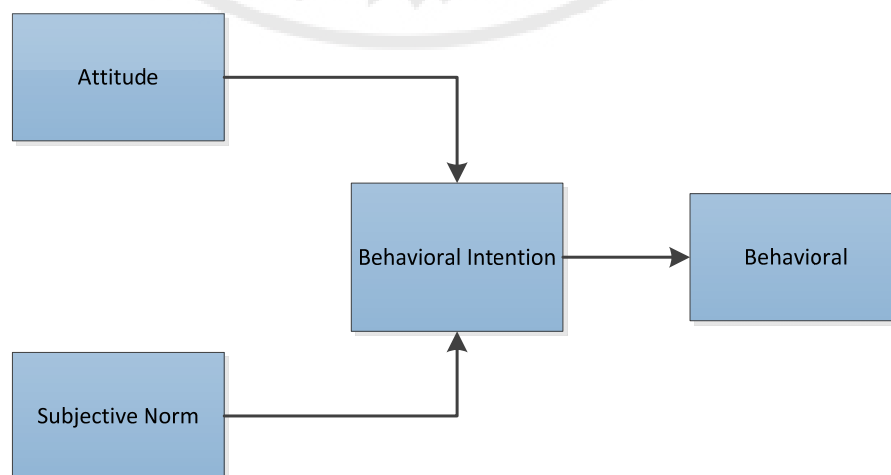
Figure 2.1 The Model of the relationship between the theories of TRA.
