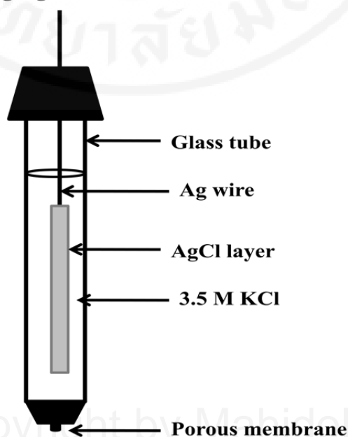
Ag/AgCl electrode
