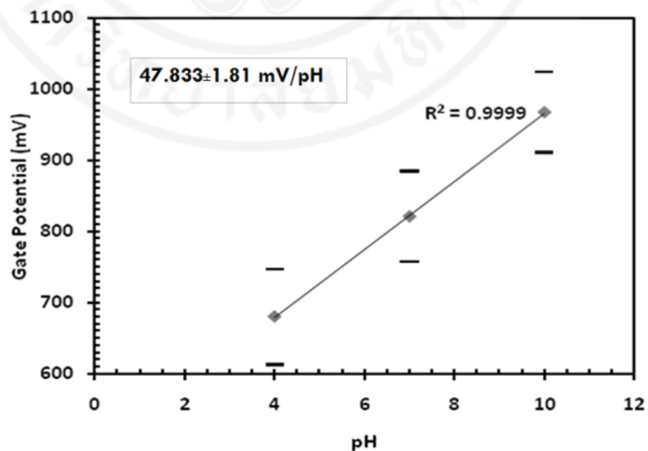
Figure 5.1 Gate potential of ISFET response to various pH solutions. The graph represents the gate potential vs. different pH. All analyses were carried out with n=10 and error bars represent \pm 1 \text{ SD} .
