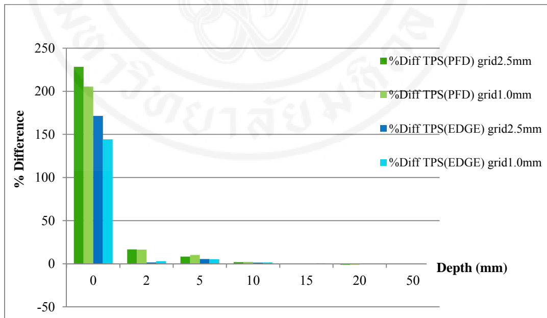
Figure 5.9. The comparison of the percentage difference of EBT 2 film measurement and both of TPS (PFD and EDGE) calculations in direct angle technique for field size of 10 × 10 cm 2 .
