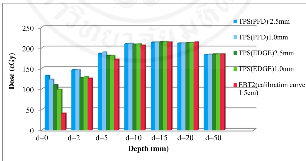
Figure 5.7. The absolute point dose at the central axis of beam of both TPS (PFD,EDGE TM ) calculation using grid size 2.5 and 1mm compared the EBT2 film measurement for field size of 10×10 cm 2 .
