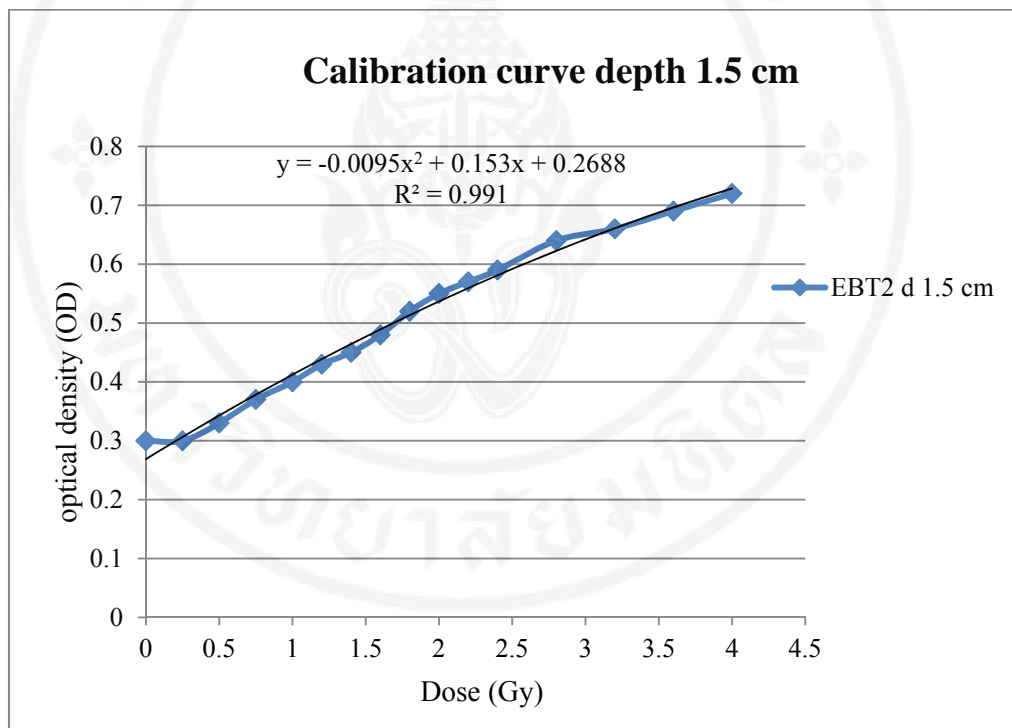
Figure 5.4 The calibration curve of EBT2 film for 6 MV photon beams, 10x10 cm 2 open field size at depth of 1.5 cm, 100 cm SAD technique.
