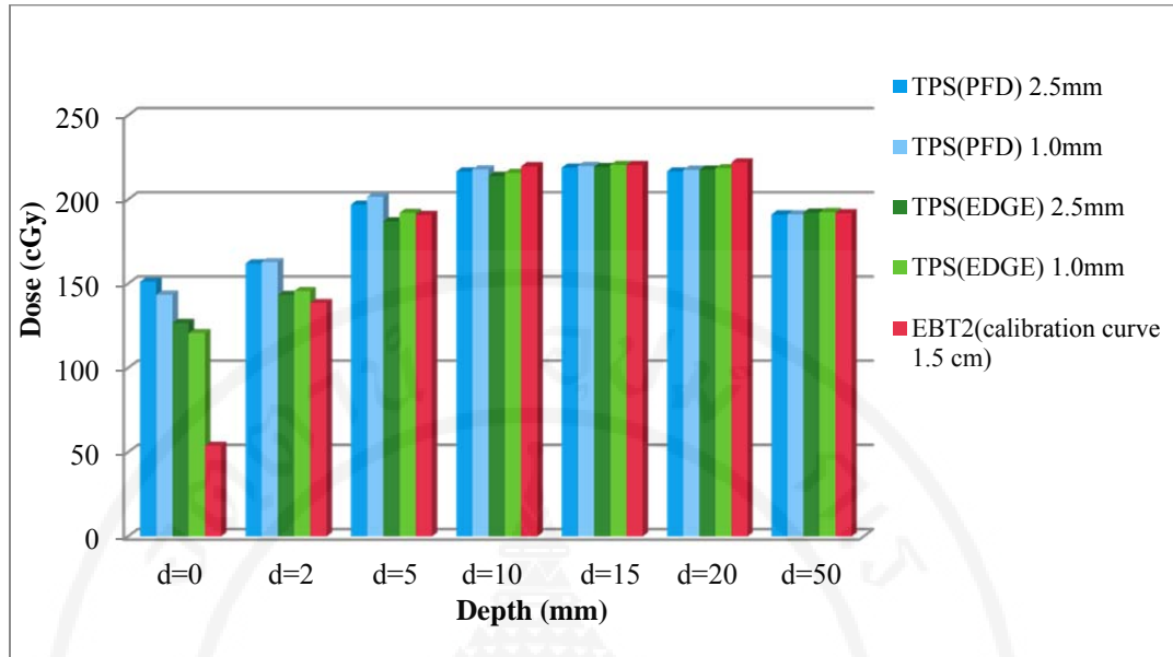
Figure 5.8. The absolute point dose at the central axis of beam of both TPS (PFD,EDGE™) calculation using grid size 2.5 and 1mm compare the EBT2 film measurement for field size of 15×15 cm 2 .
