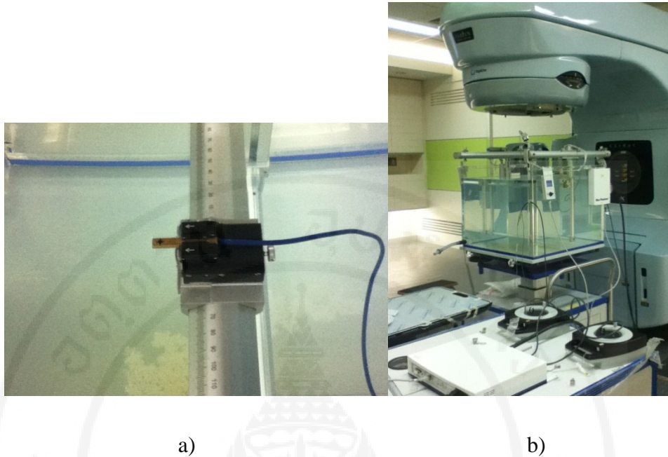
Figure 4.12 Setup the EDGE™ detector at the surface (a) and the Blue phantom 2 was setup to measure the depth doses with Variance ClinacIX linear accelerator (b)
