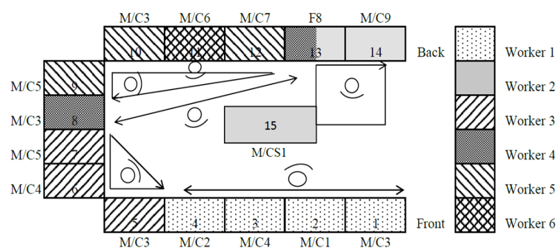
Figure 4.1 An exemplified result of case study's 36 tasks ( \alpha = 5\% \text{APT} ) on the Shared-machine U-Shaped assembly line layout
