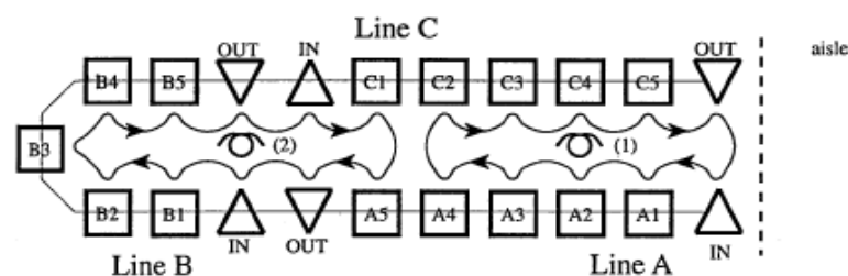
Figure 2.3 Multi-lines in a single U: Three lines in a single U (Miltenburg, 2001)
