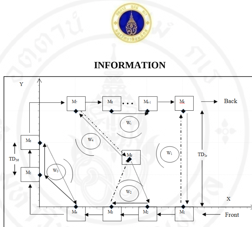
Figure A.1: The Model of Shared-machine U-shaped assembly line
