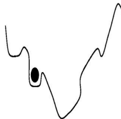
Figure 2.6(b) Problem with many relative minimum
