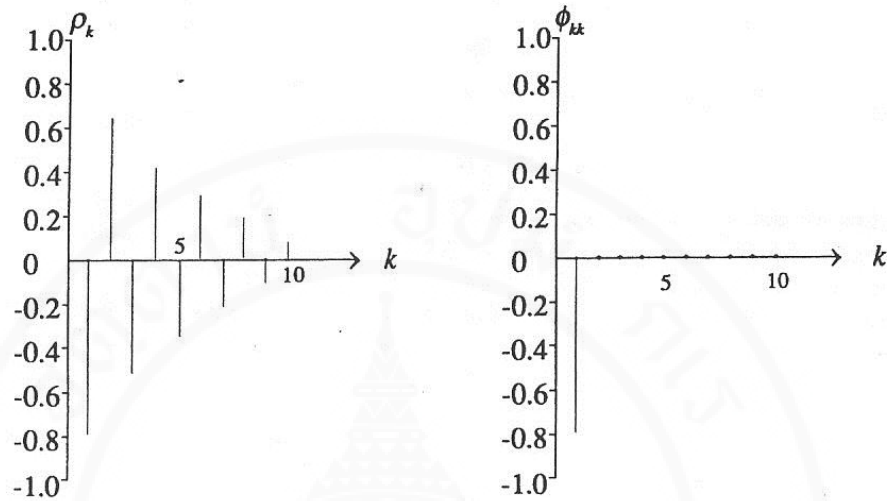
Figure A.2 ACF and PACF correlogram for ARMA(1,0) (cont.)
