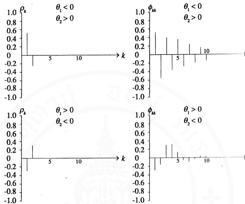
Figure A.5 ACF and PACF correlogram for ARMA(0,2) (cont.)
