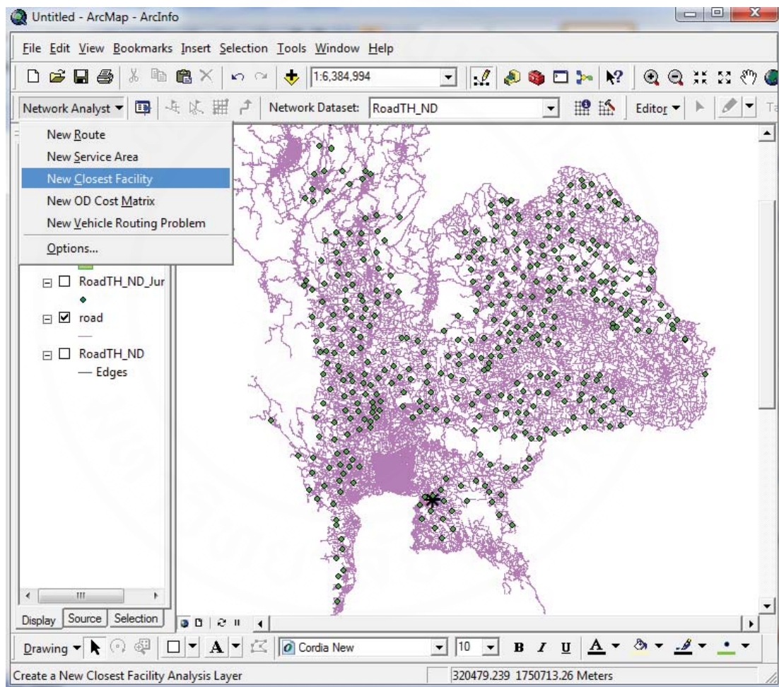
Figure C.2 Using New Closest Facility function of Network Analyst
