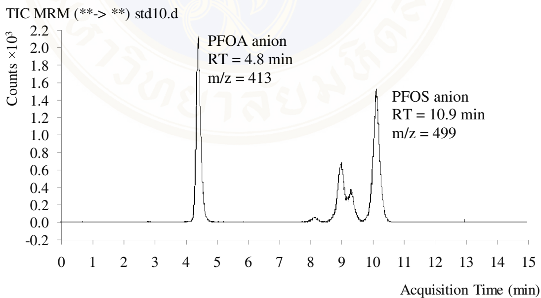
Figure 4.3 Mass Chromatographs of PFOS and PFOA at 10 \mu\text{g/L}
