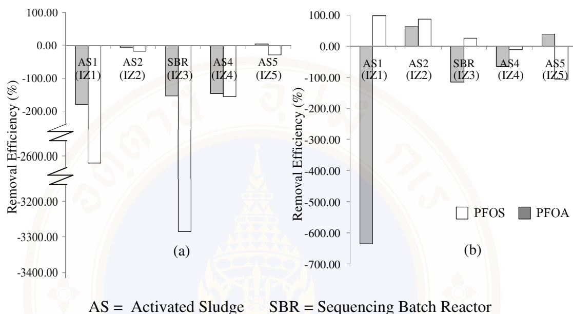
Figure 4. 20 Removal efficiency of PFOS and PFOA in central wastewater treatment plants (a) aqueous phase (b) particulate phase
