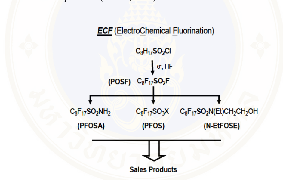
Figure 2.5 Electrochemical fluorination (ECF) process schematic.
