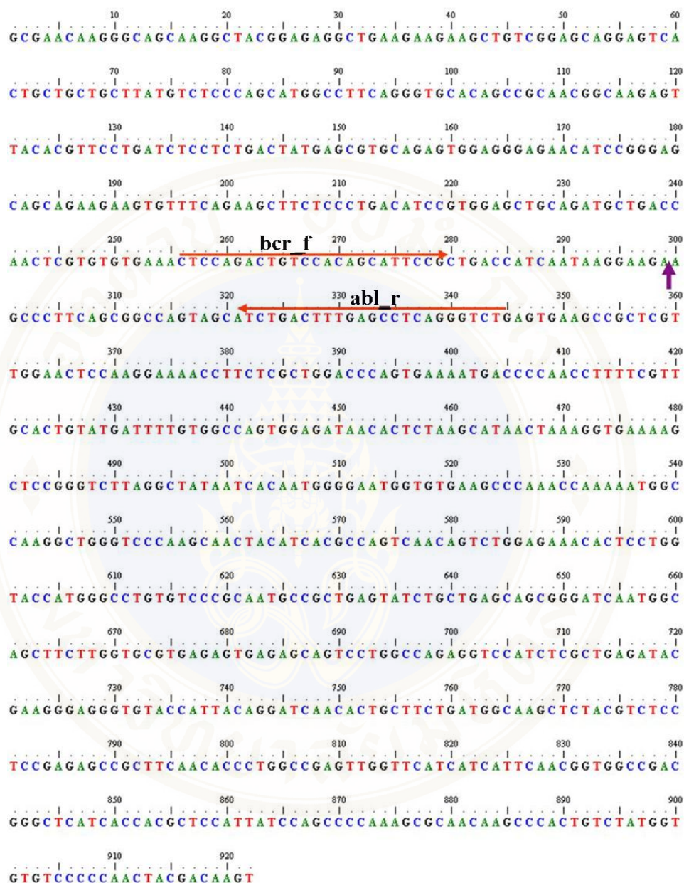
Figure 4.1 Reference nucleotide sequences of BCR-ABL fusion cDNA. The break point is indicated by a vertical purple arrow. Arrows indicate the 5' to 3' direction of the primers ( bcr_f and abl_r ). The PCR amplification of exon 13 of BCR and exon 2 of ABL gene (Figure 4.1A) and of exon 14 of BCR and exon 2 of ABL gene (Figure 4.1B) correspond to B2A2 and B3A2 variants, respectively.
