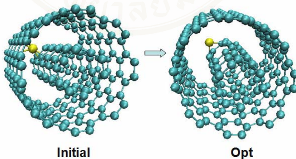
Figure 3.9: Adding of one Si atom.
