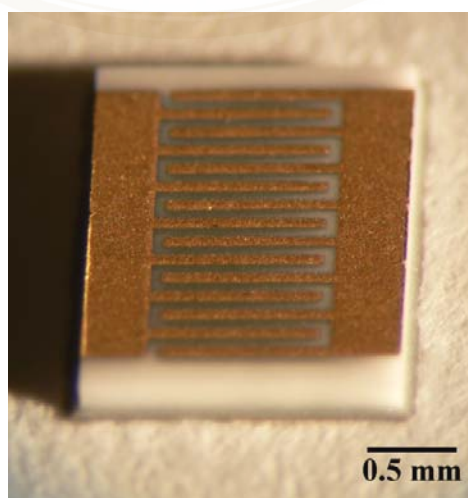
Figure 6.9: Photograph of the fabricated sensor.
