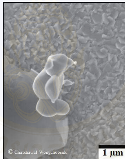
Figure 4.2: ZnO nanobear.
