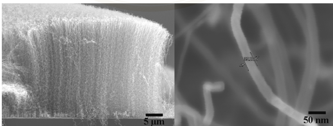
Figure 7.1: SEM images of the produced MWCNTs grown by the CVD process.
