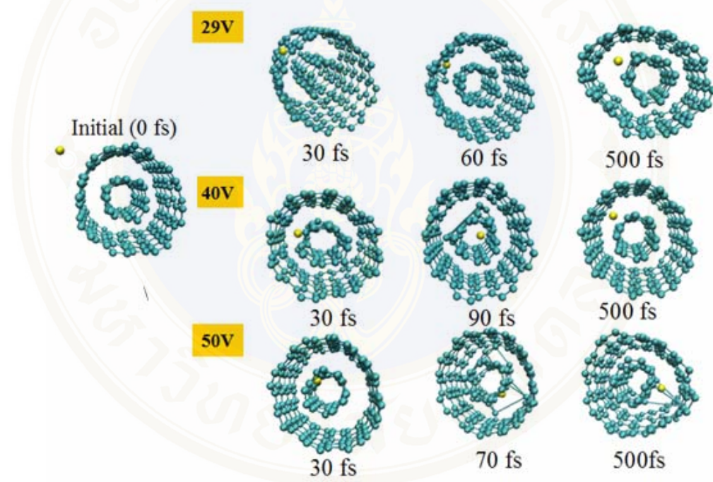
Figure 3.15: Snapshots of shooting of one Si atom at different velocity as a function of time. (Yellow color = Si atom, Green color = C atoms)
