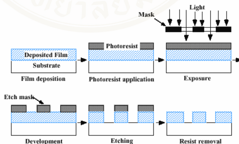
Figure 4.1: Photolithography process.
