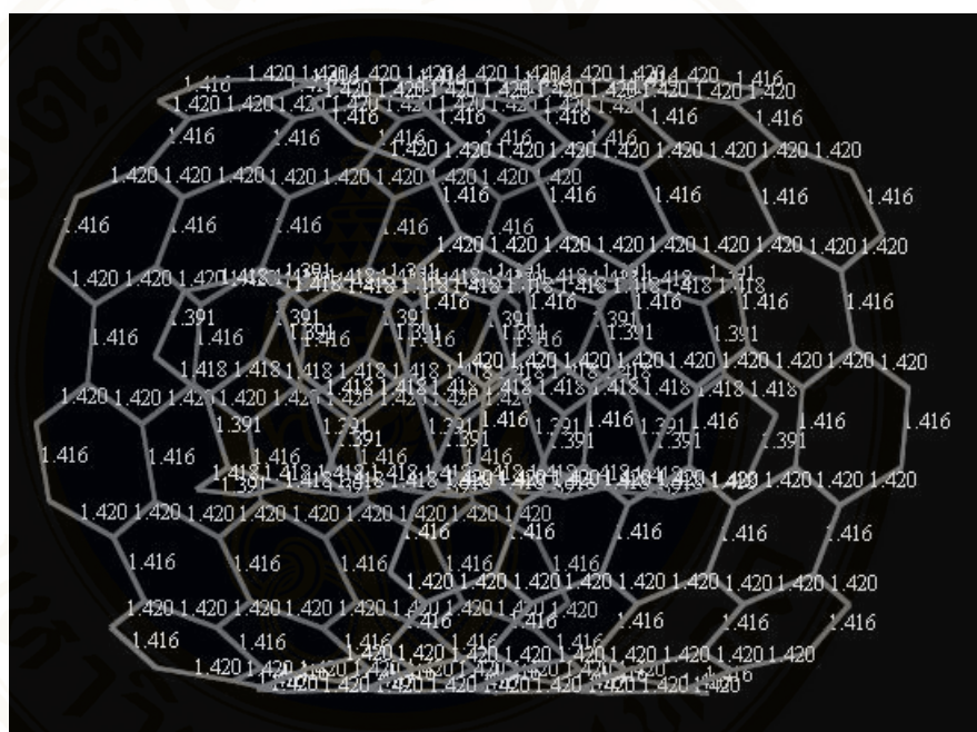
Figure 3.6: Optimized structure of armchair (3,3) in armchair (8,8).
