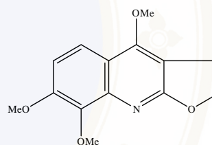
skimmianine
