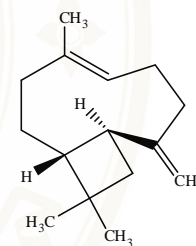
\beta -caryophyllene
