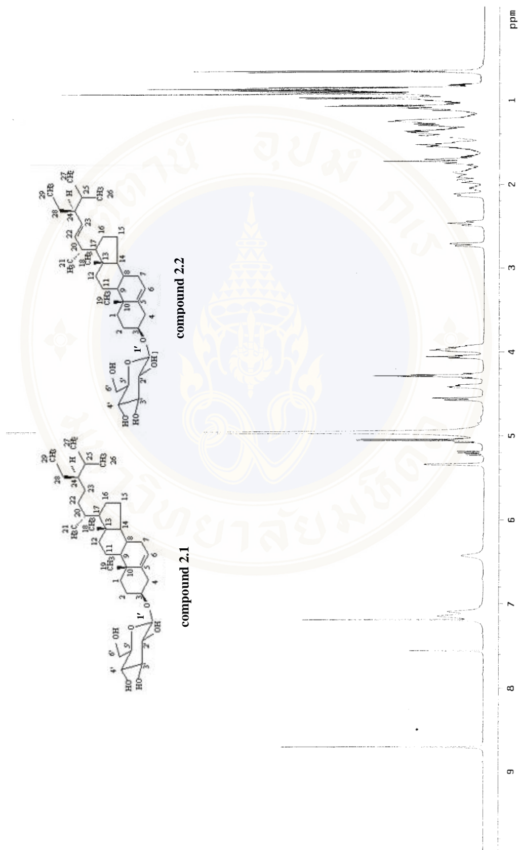
Fig. 5.17 500 MHz ^1\text{H-NMR} spectrum of compound 2 mixture in pyridine- d_5
