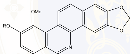
zanthoxyline
