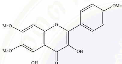
3,5,6-trihydroxy-7,4'-dimethoxyflavone
