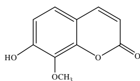
hydrangetin
