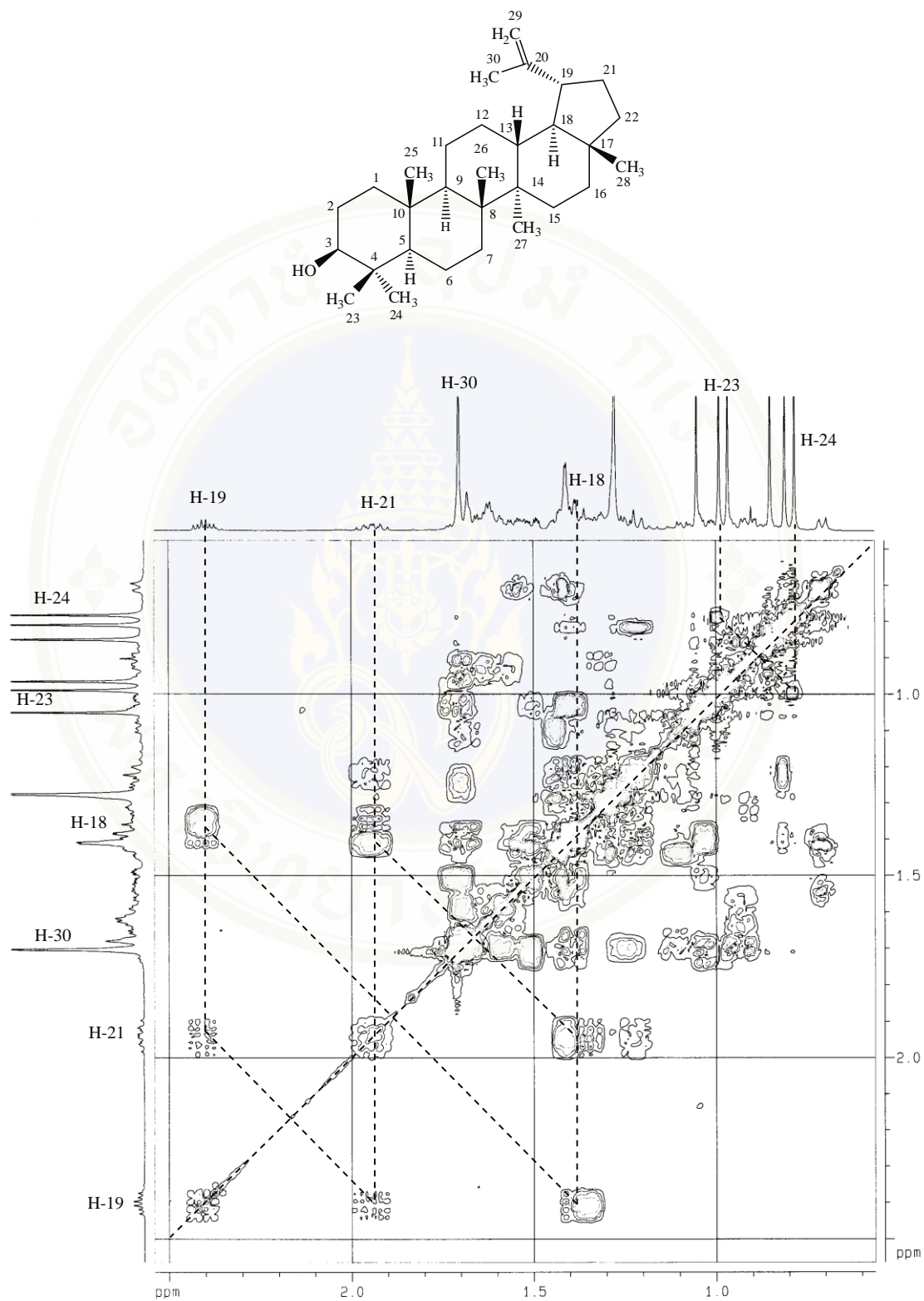
Fig. 5.38 COSY expanded spectrum of compound 3 in CDCl 3 ( \Delta\delta = 0.6 - 2.5 ppm)
