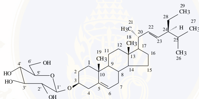
Stigmasteryl glucoside
