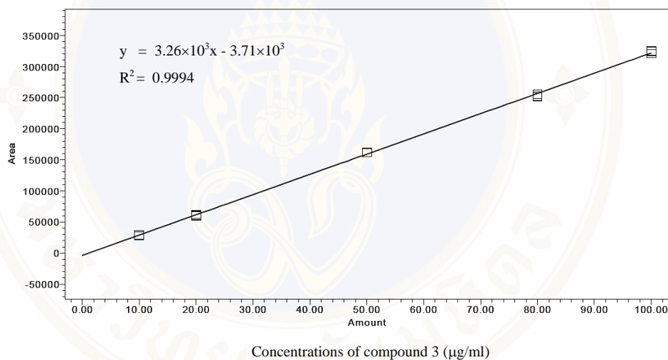
Fig 5.40 The calibration curve of compound 3
