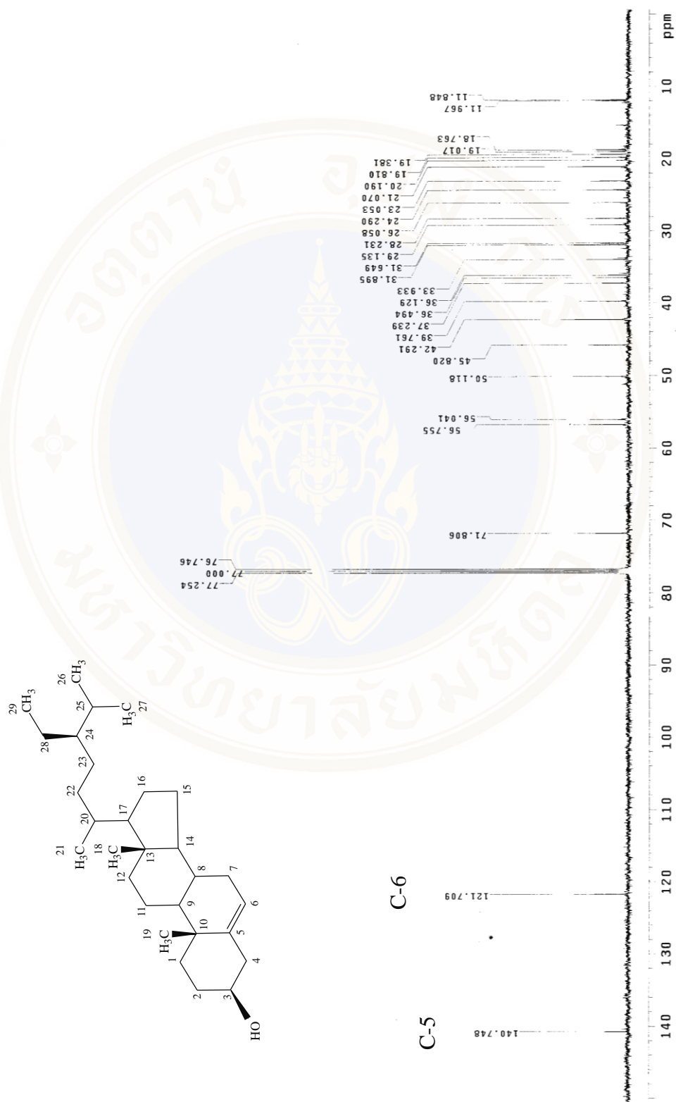
Fig. 5.6 125.7 MHz 13 C-NMR spectrum of compound 1 in CDCl 3
