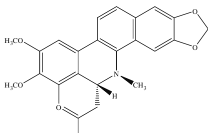
8-acetyldihydronitridine
