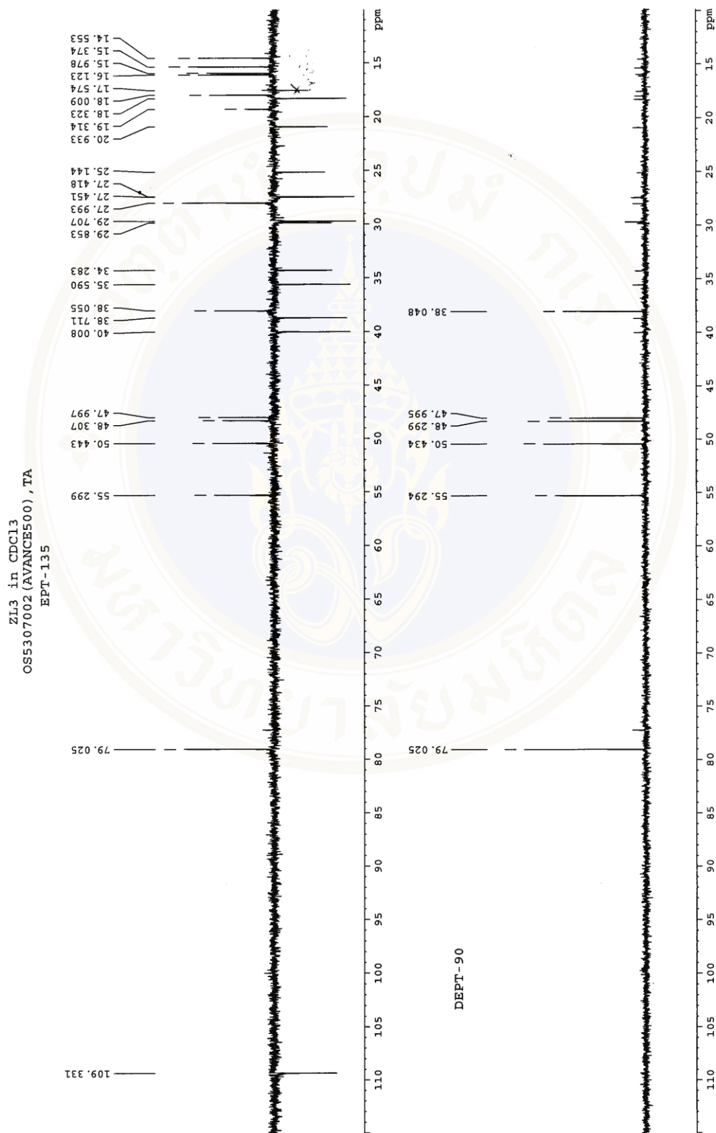
Fig. 5.25 DEPT 90 and 135 spectrum of compound 3 in CDCl 3
