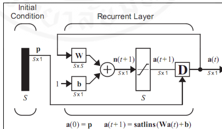
Figure 2.6 Recurrent Network
