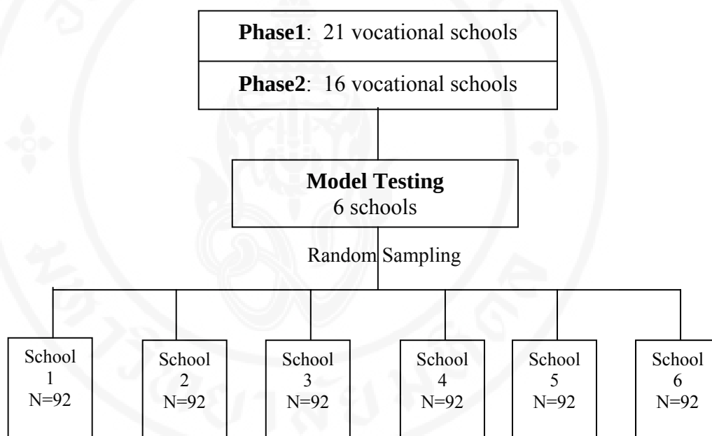
Figure 5: Sampling Scheme of Phase 2, Model Testing
