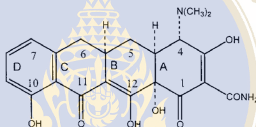
Figure 2.9 Structure of 6-deoxy-6-demethyltetracycline, the minimum tetracycline pharmacophore (50).
