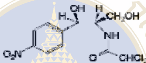
Figure 2.10 Chemical structure of chloramphenicol.
