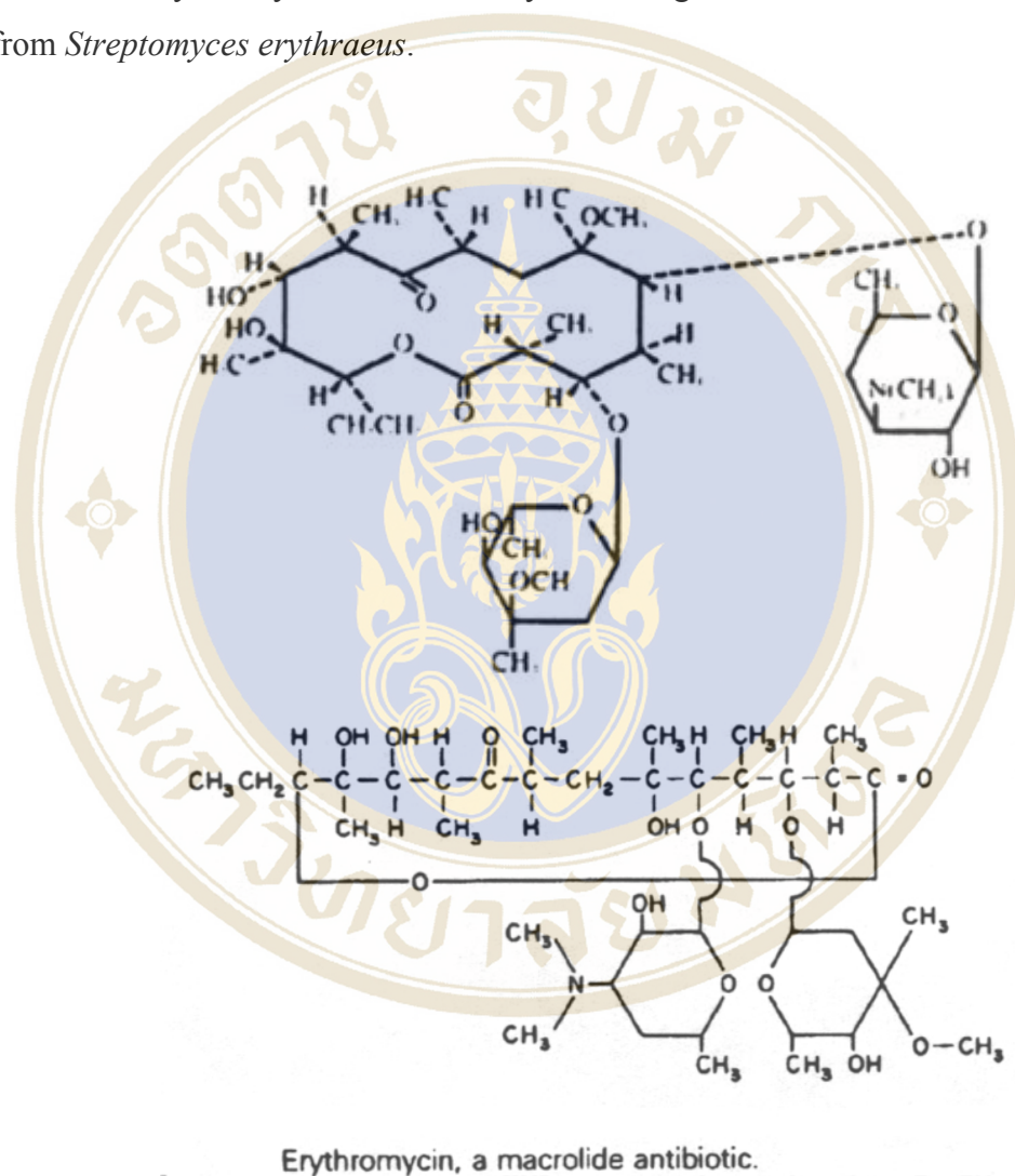
Figure 2.11 Structure of erythromycin, a macrolide antibiotic.
